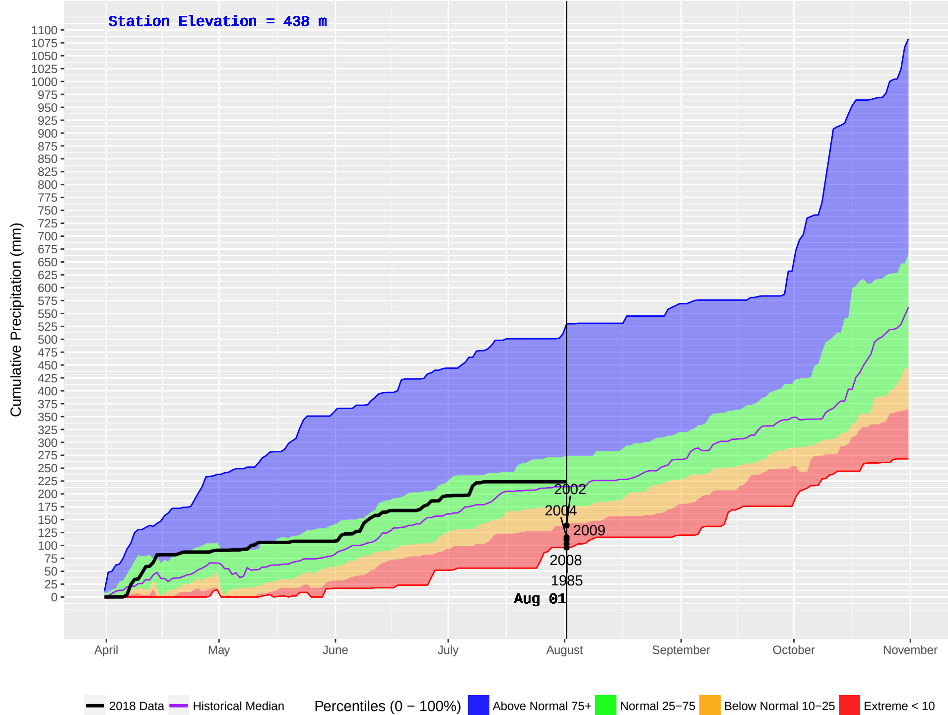
MENZIES CAMP (19) : Historical (1970–2016) and Current (2018) Daily Cumulative Precipitation
