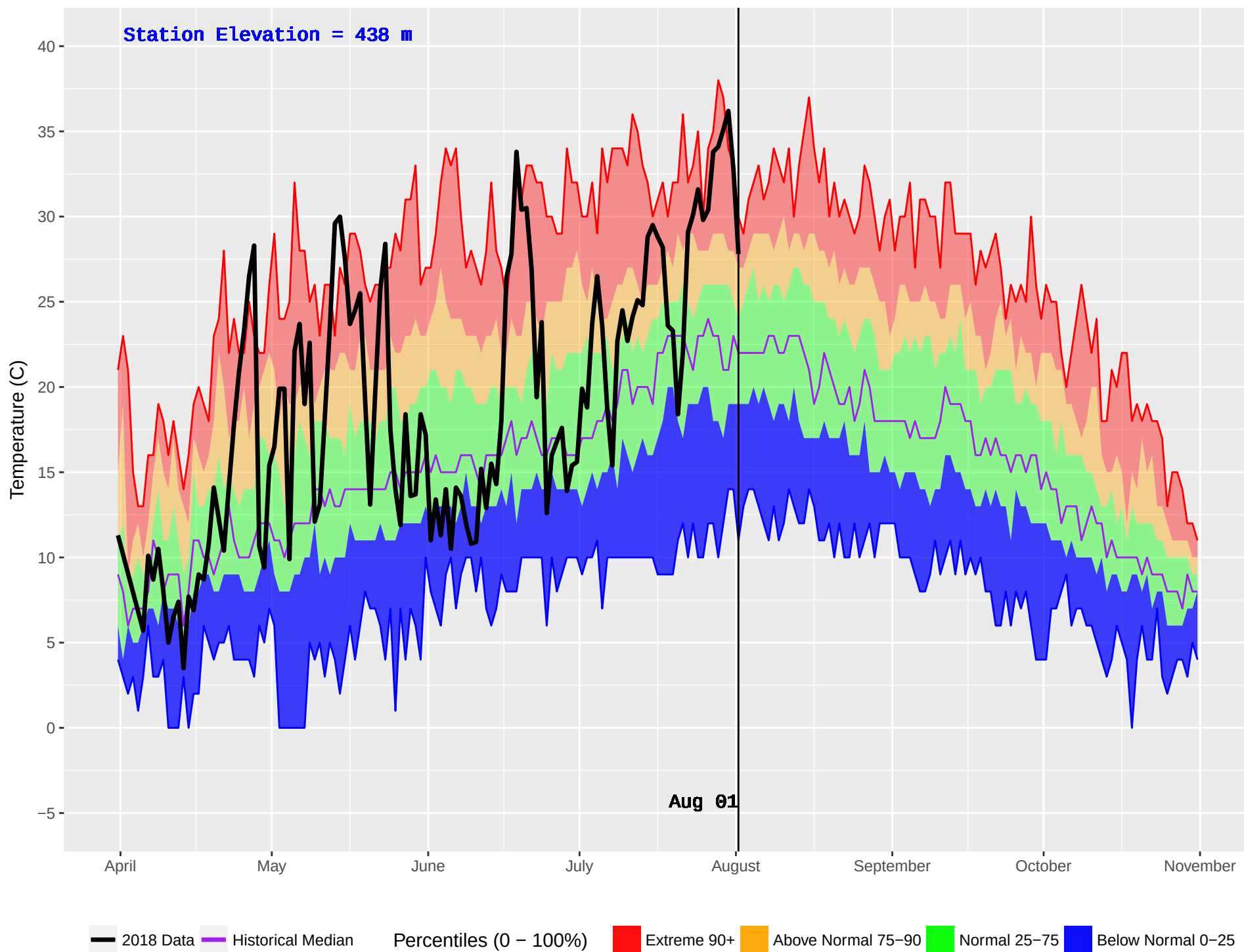
MENZIES CAMP (19) : Historical (1970–2016) and Current (2018) Daily Temperature
